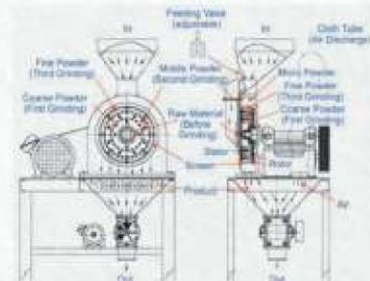
(Machine Layout)
